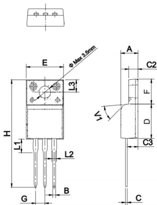
TO-220F
