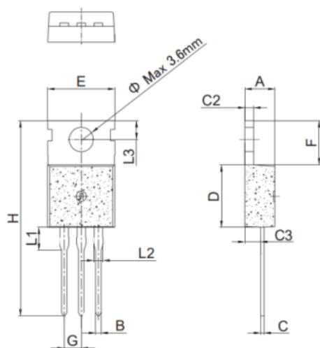
TO-220C
