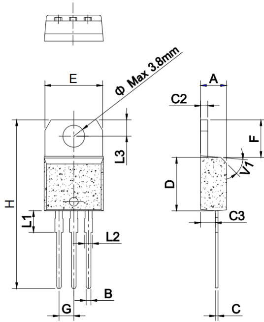
TO-220B Non-Ins
