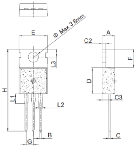
TO-220C
